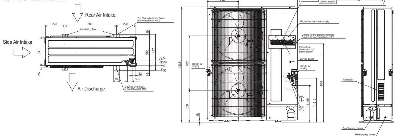
PUMY-P112/125/140VKM1/YKM1
