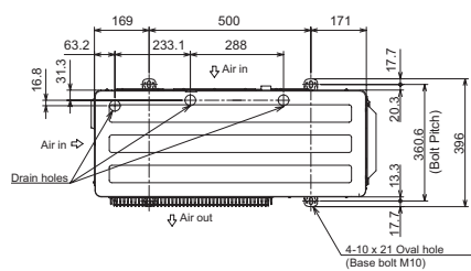
MXZ-4D72VA
