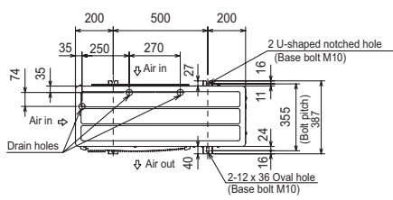
MXZ-4D83/5D102VA
